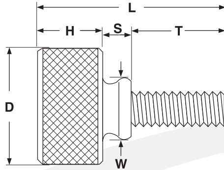
KNURLED THUMB SCREWS WITH WASHER FACE
