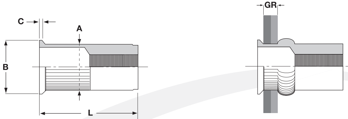
RIBBED BODY, SMALL FLANGE BLIND THREADED INSERTS
