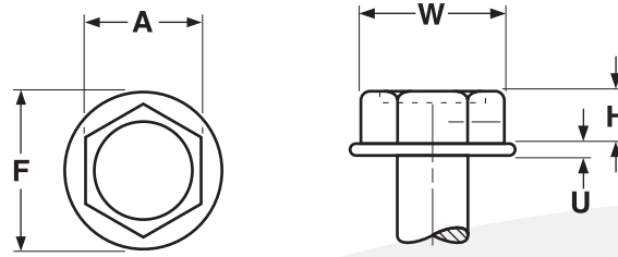
METRIC - UNSLOTTED HEX WASHER DIN 7500~D HEAD
